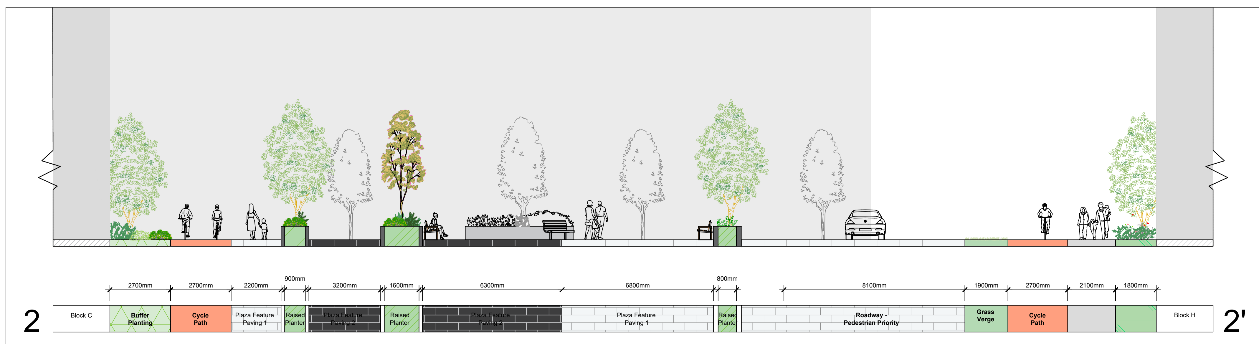
Section 2-2' sc.1:100
